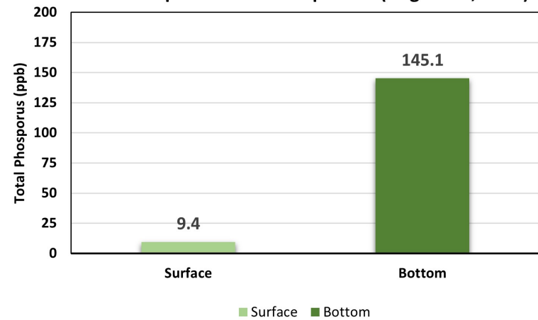
Figure 9. Wakondah Pond - Site 1 Deep Total Phosphorus inter-comparison (August 19, 2022)
