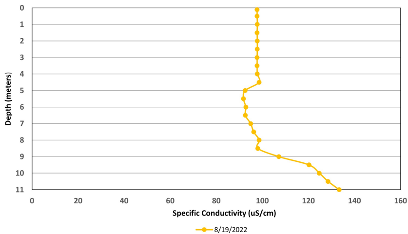
Figure 8. Wakondah Pond - Site 1 Deep Specific Conductivity Profiles (August 19, 2022)
