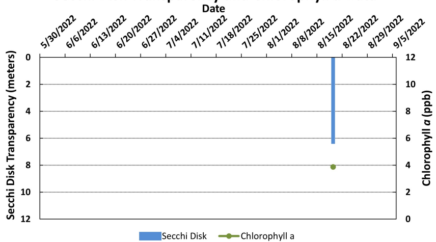
Figure 2. Wakondah Pond (2022 Seasonal Data) Secchi Disk Transparency and Chlorophyll a Data
