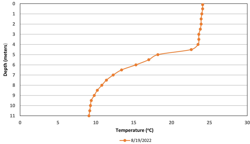
Figure 6. Wakondah Pond - Site 1 Deep Temperature Profiles (August 19, 2022)
