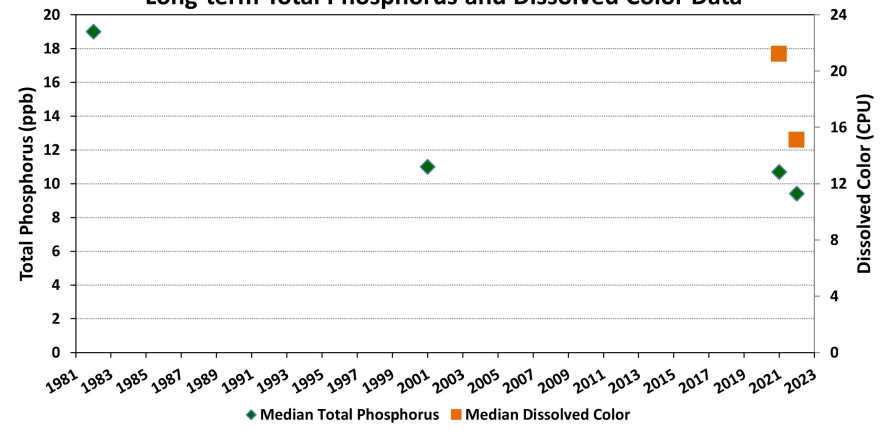
Figure 5. Wakondah Pond - Site 1 Deep (1982-2022) Long-term Total Phosphorus and Dissolved Color Data
