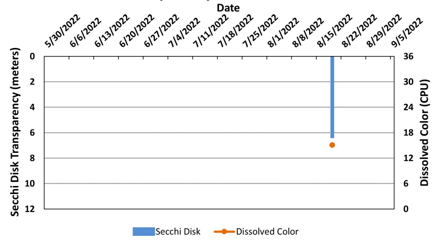
Figure 3. Wakondah Pond (2022 Seasonal Data) Secchi Disk Transparency and Dissolved Color Data
