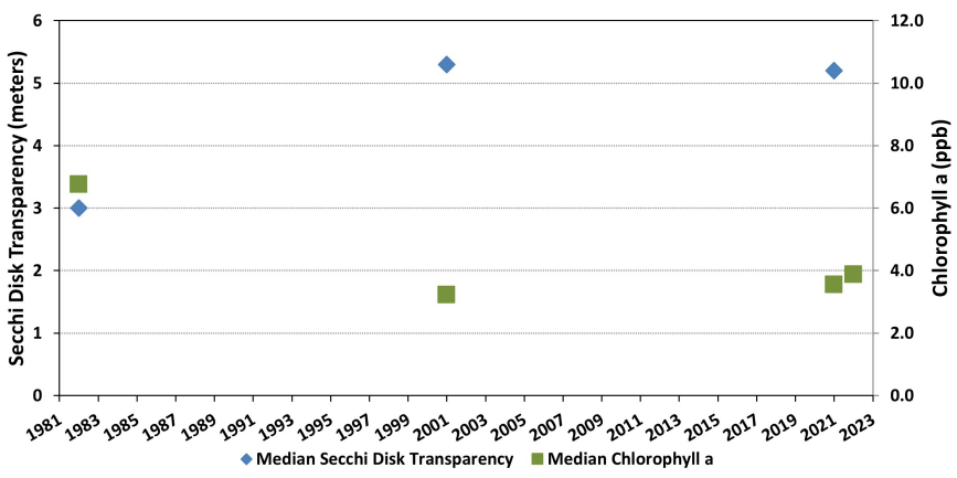
Figure 4. Wakondah Pond - Site 1 Deep (1982-2022) Long-term Secchi Disk Transparency and Chlorophyll a Data
