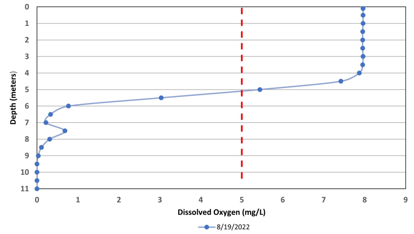
Figure 7. Wakondah Pond - Site 1 Deep Dissolved Oxygen Profiles (August 19, 2022)
