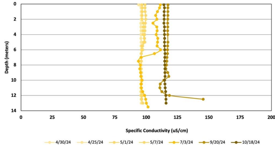
Figure 8. Lake Kanasatka - Site 1 Deep Specific Conductivity (April 25 through October 18, 2024)
