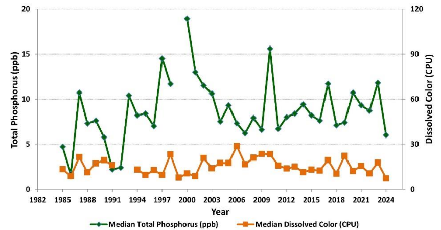
Figure 5. Lake Kanasatka - Site 1 Deep (1983-2024) Long-term Total Phosphorus and Dissolved Color Data
