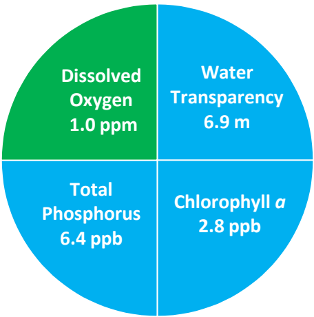
Figure 1. Lake Kanasatka Water Quality (2024)
