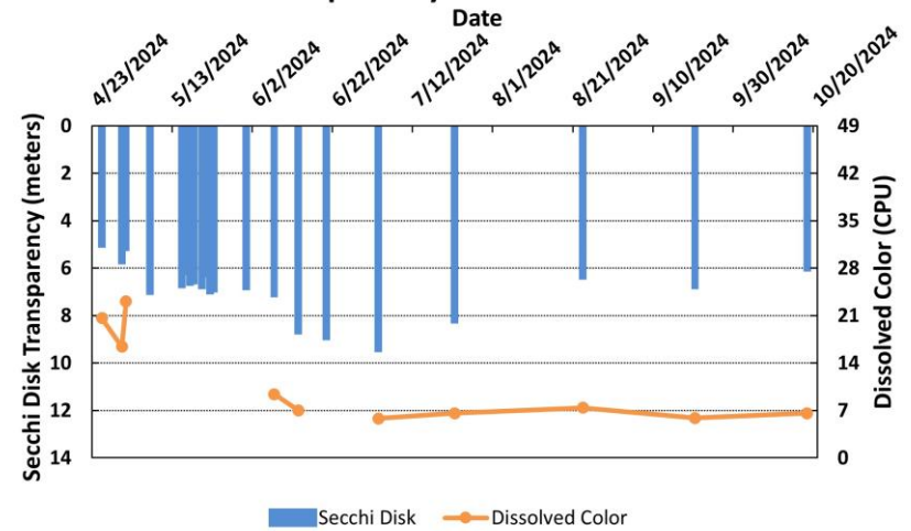
Figure 3. Lake Kanasatka (2024 Seasonal Data) Secchi Disk Transparency and Dissolved Color Data
