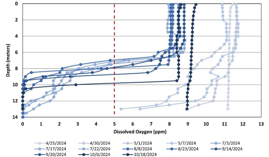
Figure 7. Lake Kanasatka - Site 1 Deep Dissolved Oxygen Profiles (April 25 through October 18, 2024)
