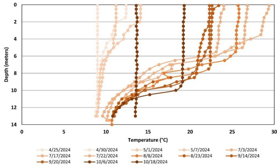
Figure 6. Lake Kanasatka - Site 1 Deep Temperature Profiles (April 25 through October 18, 2024)
