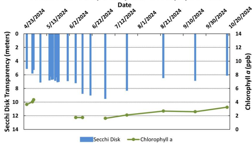
Figure 2. Lake Kanasatka (2024 Seasonal Data) Secchi Disk Transparency and Chlorophyll a Data
