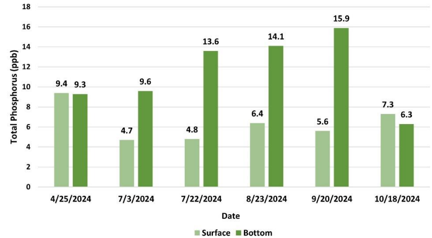
Figure 9. Lake Kanasatka- Site 1 Deep Total Phosphorus inter-comparison (April 25 through October 18, 2024)
