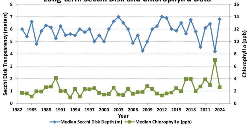
Figure 4. Lake Kanasatka - Site 1 Deep (1983-2024) Long-term Secchi Disk and Chlorophyll a Data
